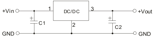
Positive Output Application Circuit
