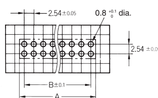
Mounting view (bottom view)
