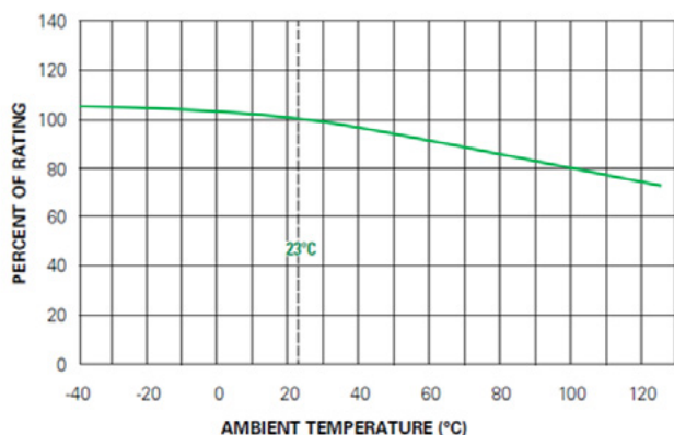
Temperature Re-rating Curve
