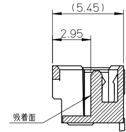
SECTION Y-Y
