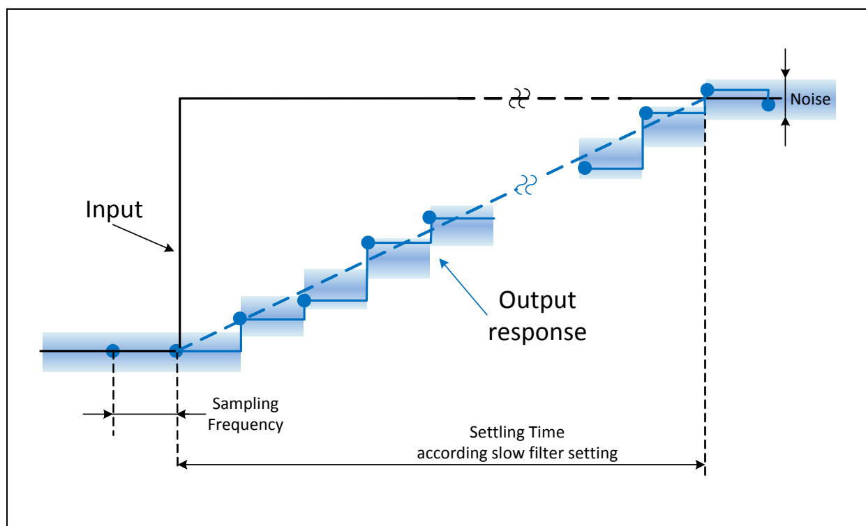
Figure 32: Step Response (fast filter off)
