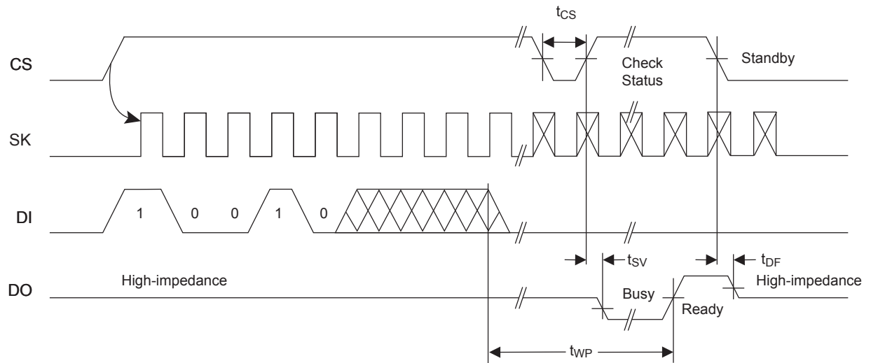
Figure 5-7. ERAL Timing
