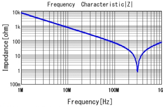
■ DE11XKX220JA4BC05F |Z| DCOV, 20degC
