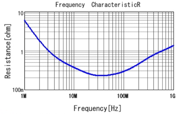
■ DE11XKX220JA4BC05F R DCOV, 20degC
