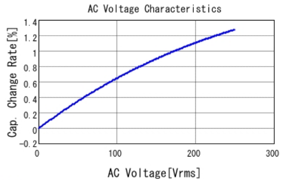
■ DE11XKX220JA4BC05F C-AC Voltage capchange, DCOV, 20.0
