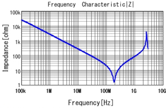
■ DE1B3KX101KA4BP01F |Z| DC0V, 20degC
