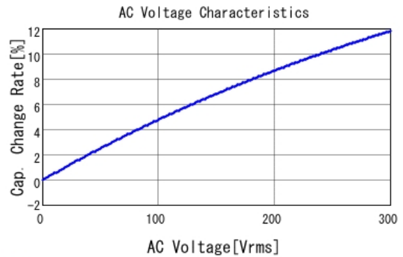
■ DE1B3KX101KA4BP01F C-AC Voltage capchange, DC0V, 20.0
