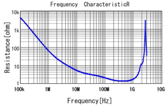
■ DE1B3KX101KA4BP01F R DC0V, 20degC
