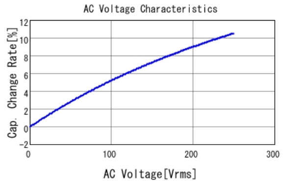
■ DE1B3KX221KA4BN01F C-AC Voltage capchange, DCOV, 20.0
