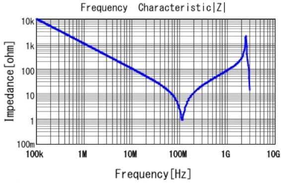
■ DE1B3KX221KA4BN01F |Z| DCOV, 20degC
