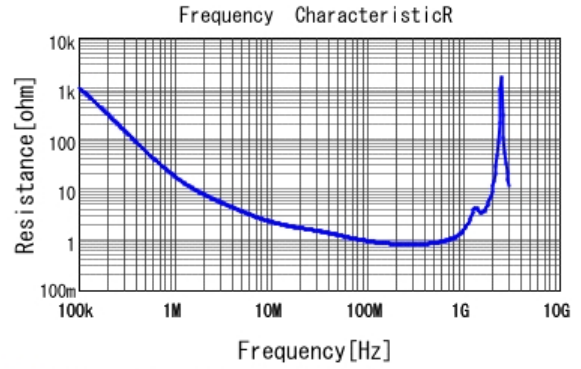
■ DE1B3KX221KA4BN01F R DCOV, 20degC
