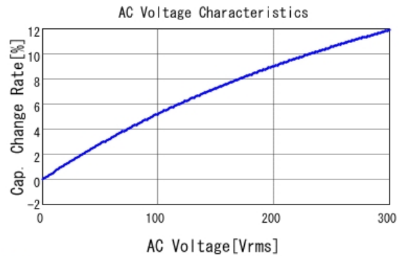
■ DE1B3KX221KA4BP01F C-AC Voltage capchange, DC0V, 20.0
