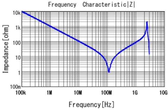
■ DE1B3KX221KA4BP01F |Z| DC0V, 20degC
