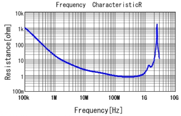
■ DE1B3KX221KA4BP01F R DC0V, 20degC
