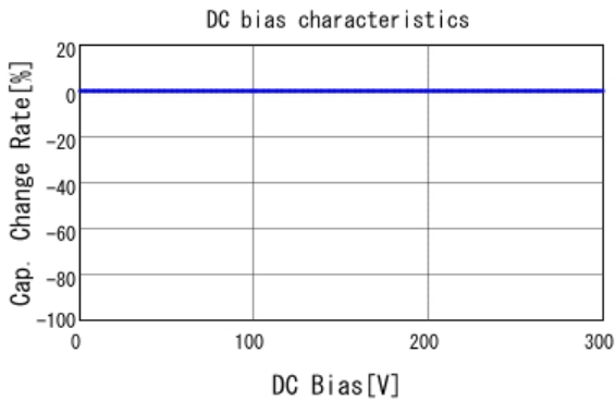
■ DE1B3KX221KA4BP01F C-DC bias capchange, 20.0degC, AC1
