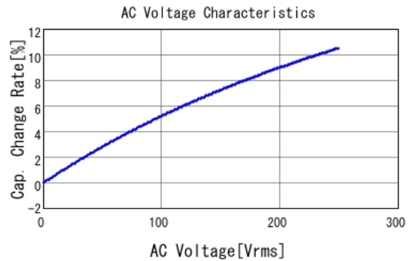
■ DE1B3KX221KN4AN01F C-AC Voltage capchange, DCOV, 20.0
