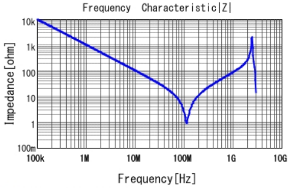
■ DE1B3KX221KN4AN01F |Z| DCOV, 20degC
