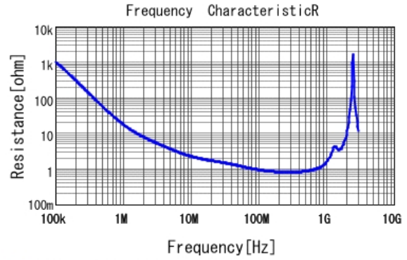
■ DE1B3KX221KN4AN01F R DCOV, 20degC
