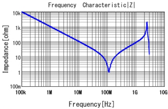
■ DE1B3KX221KN4AP01F |Z| DC0V, 20degC
