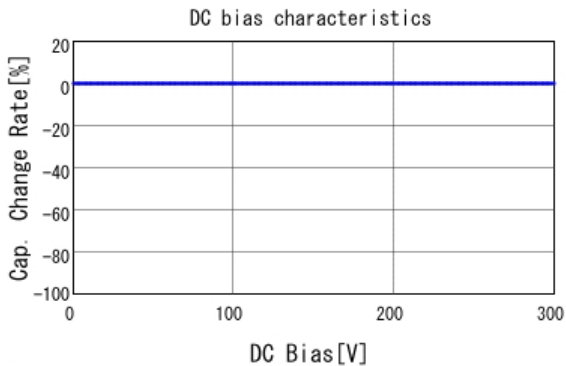
■ DE1B3KX221KN4AP01F C-DC bias capchange, 20.0degC, AC1
