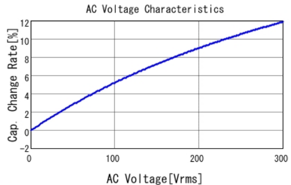
■ DE1B3KX221KN4AP01F C-AC Voltage capchange, DC0V, 20.0
