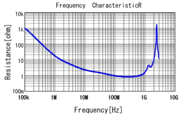
■ DE1B3KX221KN4AP01F R DC0V, 20degC
