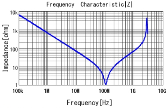
■ DE1B3KX331KA4BN01F |Z| DCOV, 20degC
