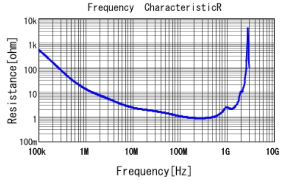
■ DE1B3KX331KA4BN01F R DCOV, 20degC
