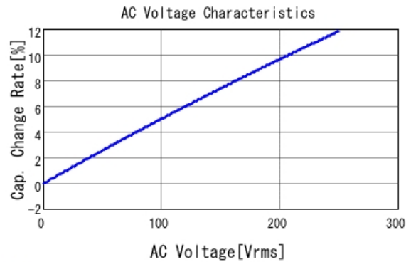
■ DE1B3KX331KA4BN01F C-AC Voltage capchange, DCOV, 20.0
