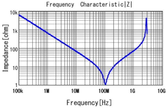
■ DE1B3KX331KN4AN01F |Z| DCOV, 20degC
