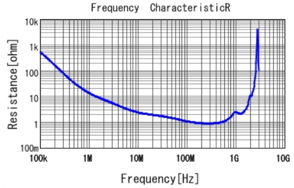
■ DE1B3KX331KN4AN01F R DCOV, 20degC
