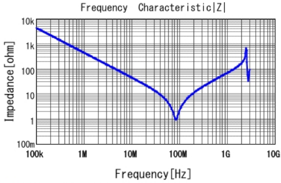
■ DE1B3KX471KA4BN01F |Z| DCOV, 20degC
