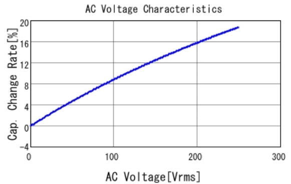
■ DE1B3KX471KN4AN01F C-AC Voltage capchange, DCOV, 20.0
