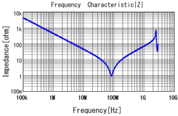
■ DE1B3KX471KN4AN01F |Z| DCOV, 20degC
