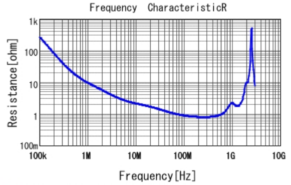
■ DE1B3KX471KN4AN01F R DCOV, 20degC
