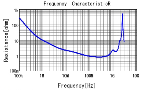
■ DE1B3KX471KN4AP01F R DCOV, 20degC
