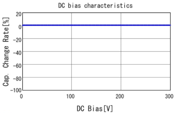
■ DE1B3KX471KN4AP01F C-DC bias capchange, 20.0degC, AC1
