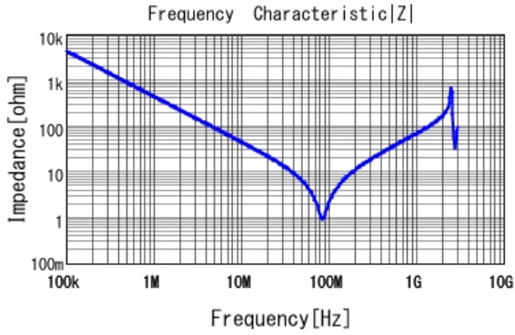
■ DE1B3KX471KN4AP01F |Z| DCOV, 20degC
