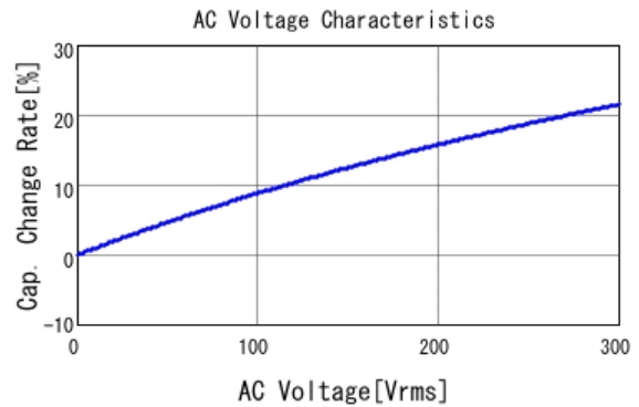
■ DE1B3KX471KN4AP01F C-AC Voltage capchange, DCOV, 20.0
