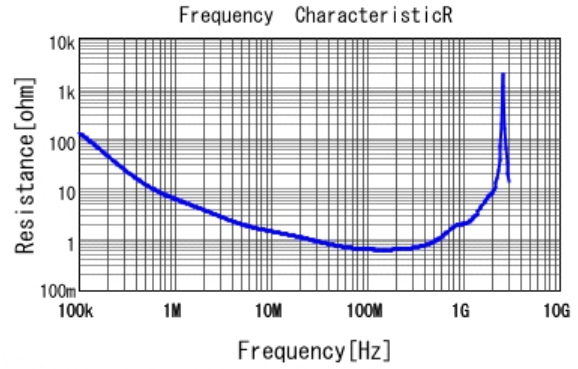
■ DE1B3KX681KA4BN01F R DCOV, 20degC
