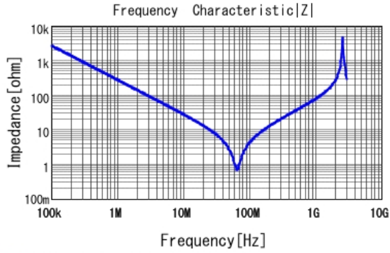
■ DE1B3KX681KA4BN01F |Z| DCOV, 20degC
