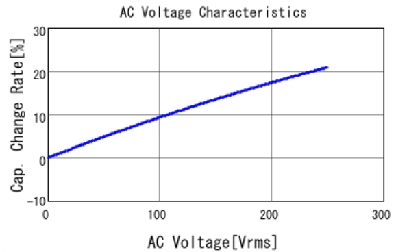
■ DE1B3KX681KA4BN01F C-AC Voltage capchange, DCOV, 20.0
