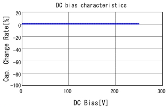
■ DE1B3KX681KA4BN01F C-DC bias capchange, 20.0degC, AC1
