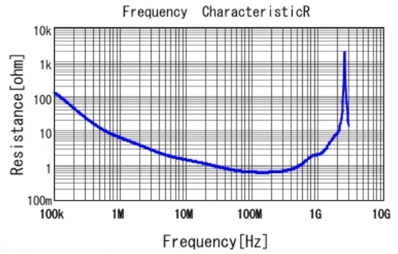
■ DE1B3KX681KA4BP01F R DCOV, 20degC
