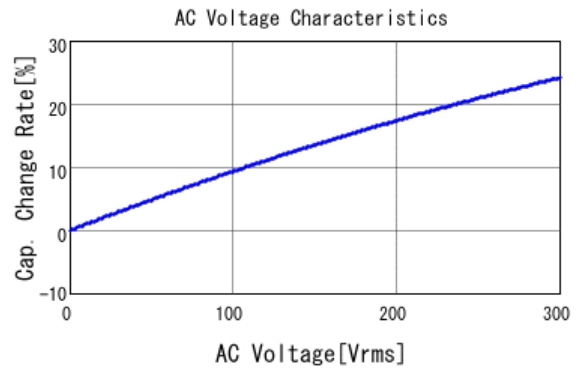
■ DE1B3KX681KA4BP01F C-AC Voltage capchange, DCOV, 20.0
