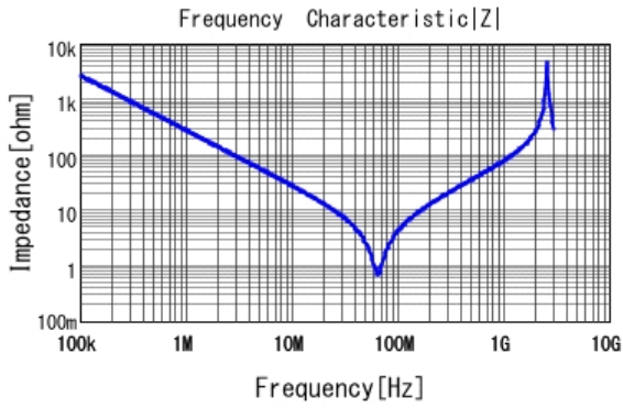
■ DE1B3KX681KA4BP01F |Z| DCOV, 20degC
