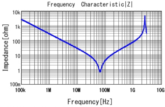
■ DE1B3KX681KN4AN01F |Z| DCOV, 20degC
