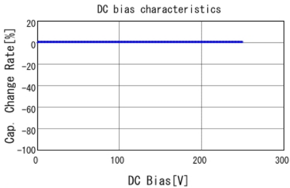
■ DE1B3KX681KN4AN01F C-DC bias capchange, 20.0degC, AC1
