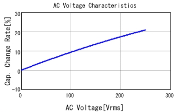
■ DE1B3KX681KN4AN01F C-AC Voltage capchange, DCOV, 20.0
