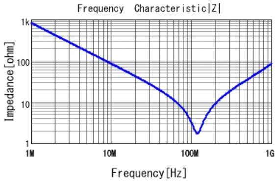
■ DE1B3RA221KA4BP01F |Z| DCOV, 20degC
