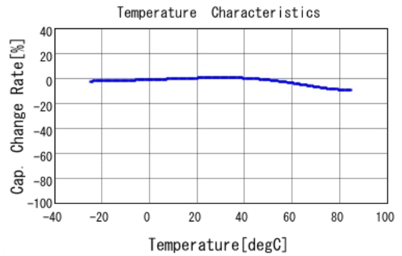
■ DE1B3RA221KA4BP01F C-Temp. capchange, DCOV, AC1Vrms
