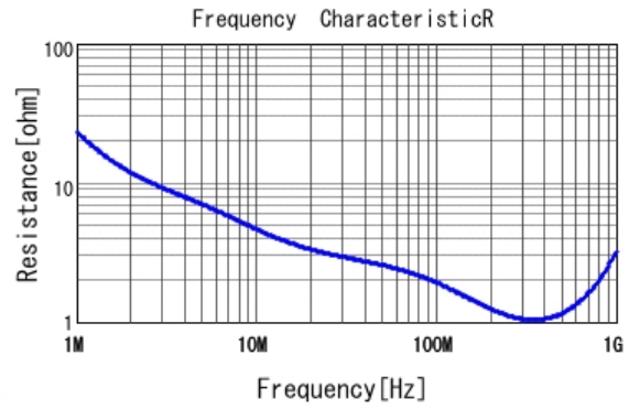
■ DE1B3RA221KA4BP01F R DCOV, 20degC
