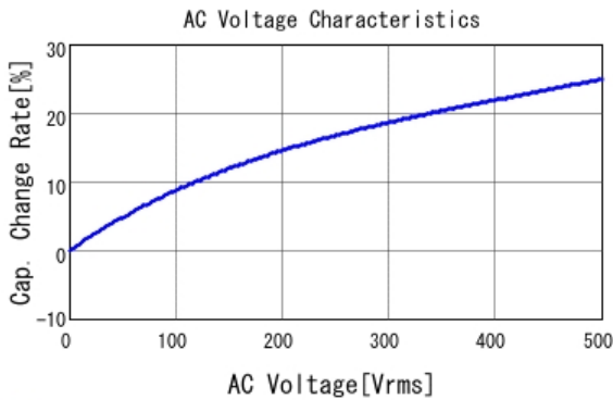
■ DE1B3RA471KJ4BQ01F C-AC Voltage capchange, DCOV, 20.0
