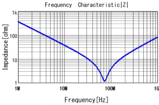
■ DE1B3RA471KJ4BQ01F |Z| DCOV, 20degC
