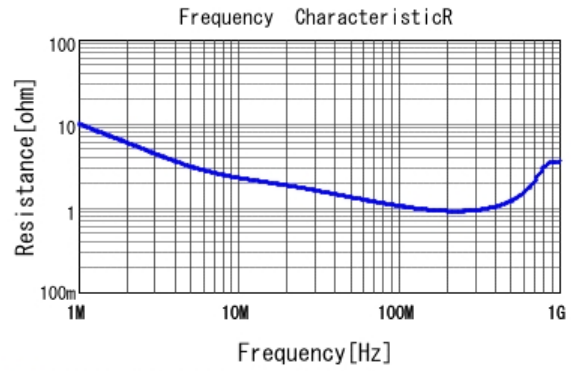
■ DE1B3RA471KJ4BQ01F R DCOV, 20degC
