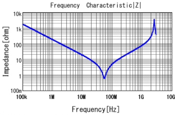
■ DE1E3KX102MA4BP01F |Z| DC0V, 20degC
