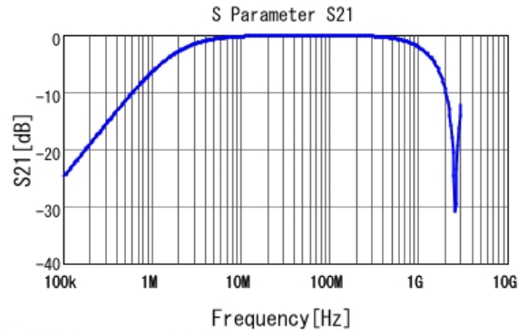
■ DE1E3KX102MA4BP01F S21 DCOV, 20degC
