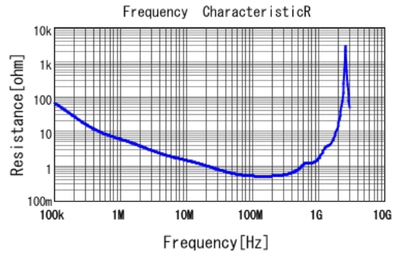
■ DE1E3KX102MA4BP01F R DC0V, 20degC
