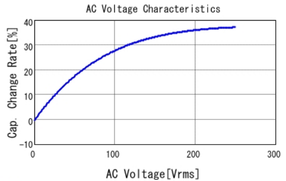
■ DE1E3KX102MB4BN01F C-AC Voltage capchange, DCOV, 20.0
