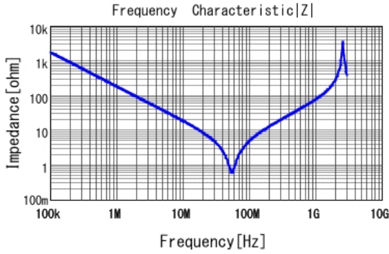
■ DE1E3KX102MB4BN01F |Z| DCOV, 20degC
