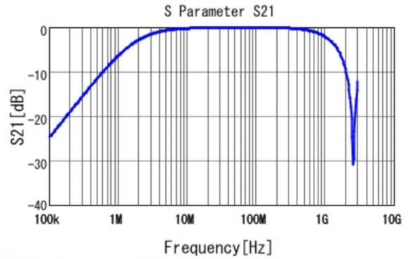
■ DE1E3KX102MN4AN01F S21 DCOV, 20degC
