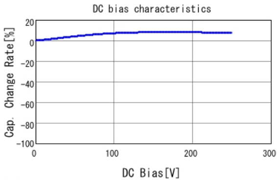
■ DE1E3KX102MN4AN01F C-DC bias capchange, 20.0degC, AC1
