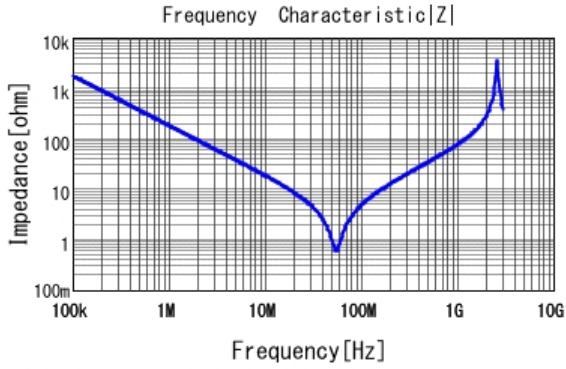
■ DE1E3KX102MN4AN01F |Z| DCOV, 20degC
