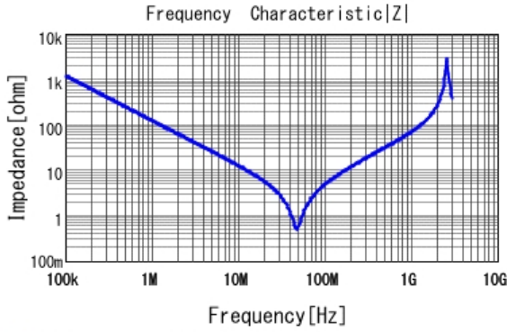
■ DE1E3KX152MA4BN01F |Z| DCOV, 20degC
