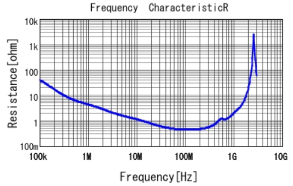
■ DE1E3KX152MA4BN01F R DCOV, 20degC
