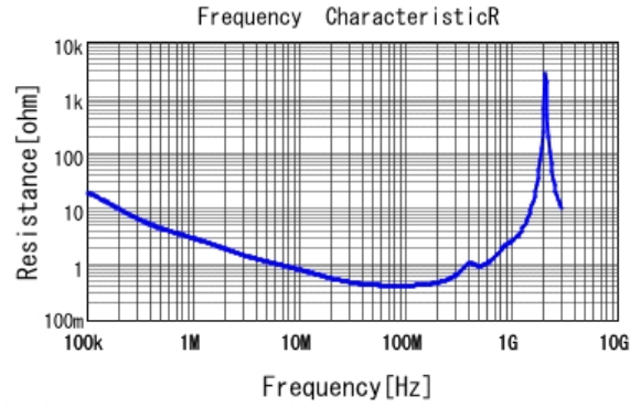
■ DE1E3KX222MB4BN01F R DCOV, 20degC
