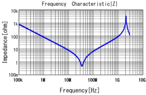
■ DE1E3KX222MB4BN01F |Z| DCOV, 20degC
