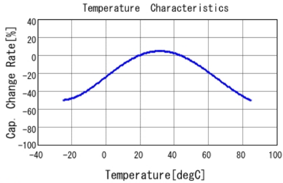
■ DE1E3KX222MB4BN01F C-Temp. capchange, DCOV, AC1Vrms
