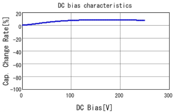
■ DE1E3KX222MB4BN01F C-DC bias capchange, 20.0degC, AC1
