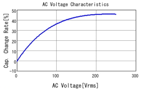
■ DE1E3KX222MB4BN01F C-AC Voltage capchange, DCOV, 20.0
