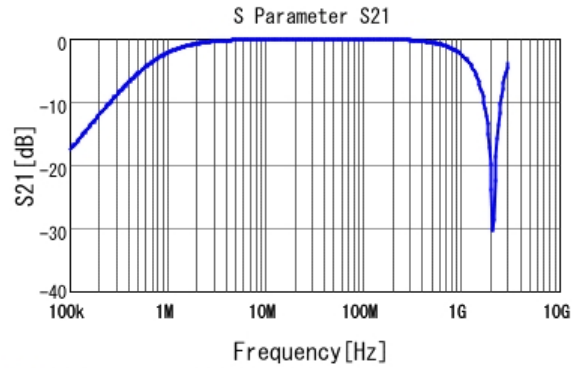
■ DE1E3KX222MN4AN01F S21 DCOV, 20degC
