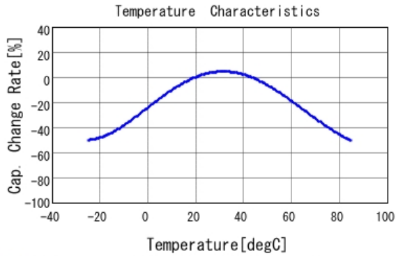
■ DE1E3KX222MN4AN01F C-Temp. capchange, DCOV, AC1Vrms
