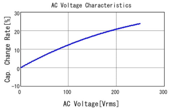
■ DE1E3KX332MN4AN01F C-AC Voltage capchange, DCOV, 20.0
