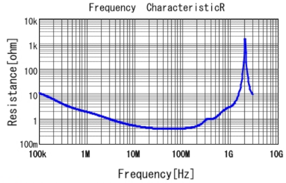
■ DE1E3KX332MN4AN01F R DCOV, 20degC
