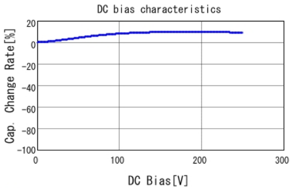
■ DE1E3KX472MN4AN01F C-DC bias capchange, 20.0degC, AC1
