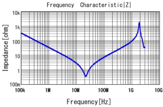
■ DE1E3KX472MN4AN01F |Z| DCOV, 20degC
