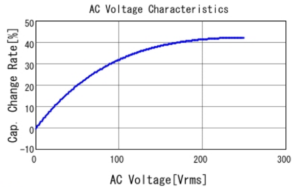
■ DE1E3KX472MN4AN01F C-AC Voltage capchange, DCOV, 20.0
