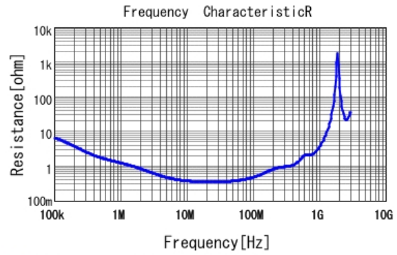
■ DE1E3KX472MN4AN01F R DCOV, 20degC
