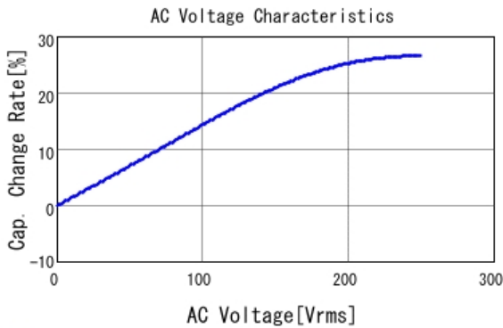
■ DE1E3RA222MA4BN01F C-AC Voltage capchange, DCOV, 20.0
