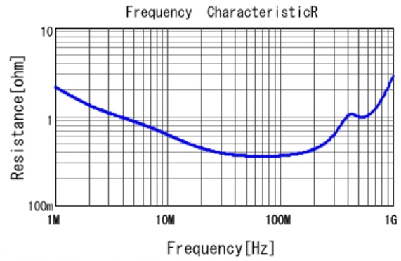
■ DE1E3RA222MJ4BN01F R DCOV, 20degC
