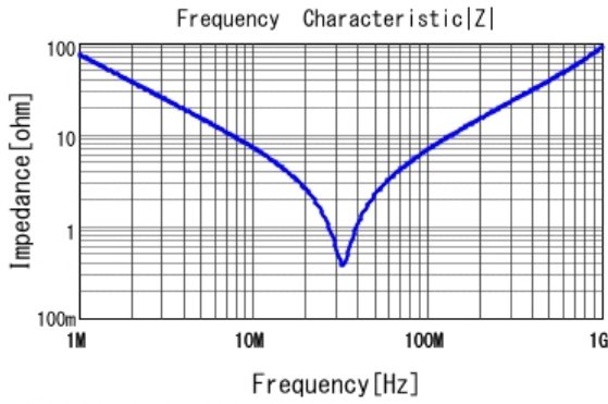
■ DE1E3RA222MJ4BN01F |Z| DCOV, 20degC
