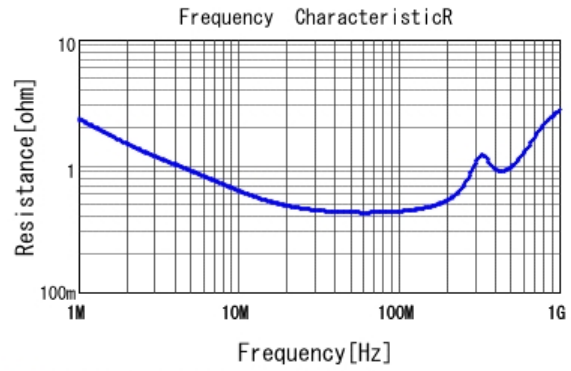
■ DE1E3RA222MJ4BQ01F R DCOV, 20degC
