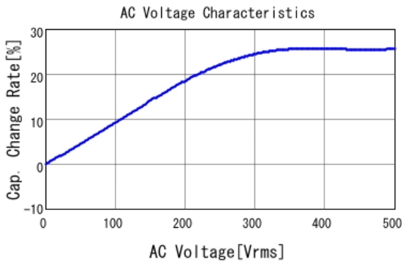
■ DE1E3RA222MJ4BQ01F C-AC Voltage capchange, DCOV, 20.0
