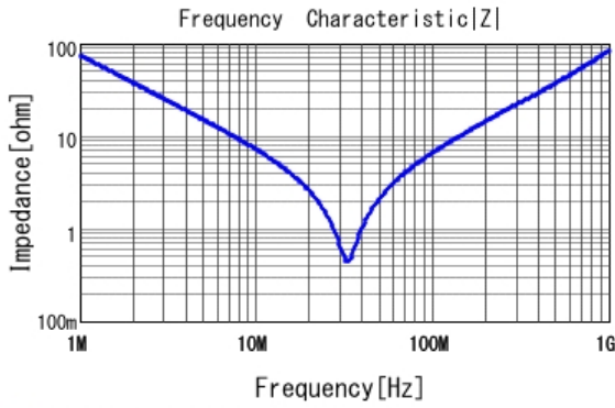
■ DE1E3RA222MJ4BQ01F |Z| DCOV, 20degC
