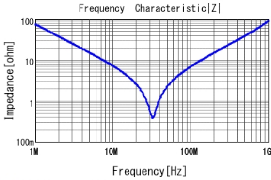
■ DE1E3RA222MN4AN01F |Z| DCOV, 20degC
