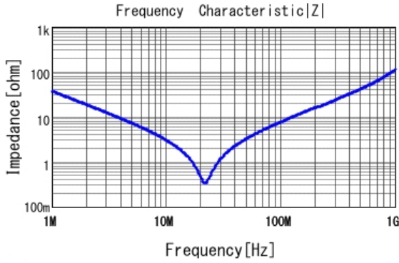
■ DE1E3RA472MJ4BQ01F |Z| DCOV, 20degC
