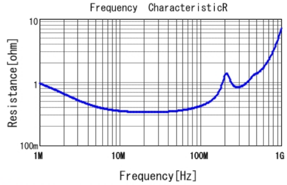
■ DE1E3RA472MJ4BQ01F R DCOV, 20degC
