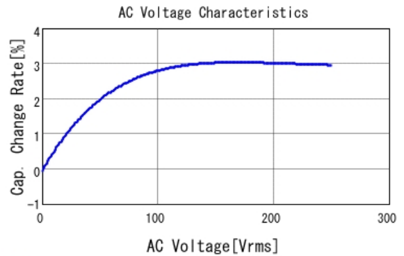
■ DE21XKY470JA2BM01F C-AC Voltage capchange, DCOV, 20.0
