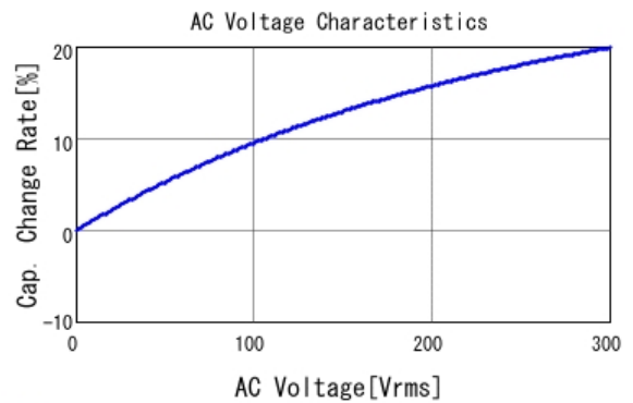
■ DE2B3KY101KA3BU02F C-AC Voltage capchange, DCOV, 20.0
