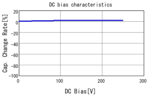
■ DE2B3KY221KA3BM02F C-DC bias capchange, 20.0degC, AC1
