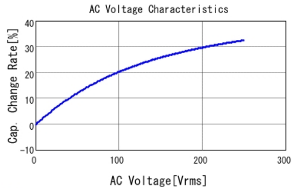
■ DE2B3KY221KA3BM02F C-AC Voltage capchange, DCOV, 20.0
