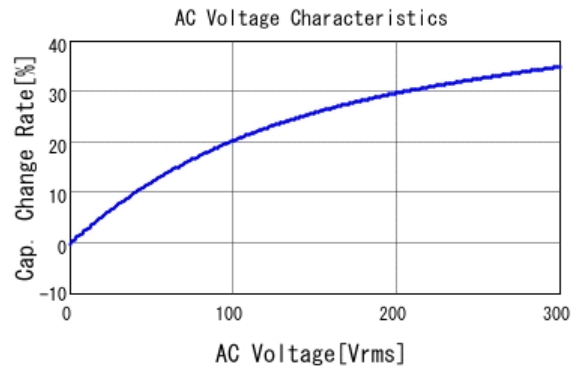
■ DE2B3KY221KB3BU02F C-AC Voltage capchange, DCOV, 20.0
