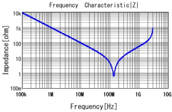
■ DE2B3KY221KB3BU02F |Z| DCOV, 20degC
