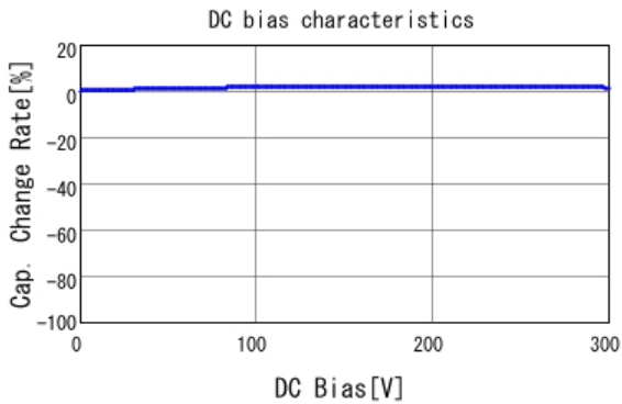
■ DE2B3KY221KB3BU02F C-DC bias capchange, 20.0degC, AC1
