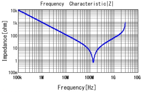
■ DE2B3KY221KN3AM02F |Z| DCOV, 20degC
