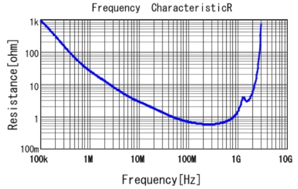
■ DE2B3KY221KN3AM02F R DCOV, 20degC
