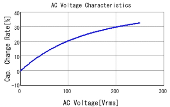
■ DE2B3KY221KN3AM02F C-AC Voltage capchange, DCOV, 20.0
