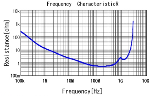
■ DE2B3KY471KA3BM02F R DCOV, 20degC
