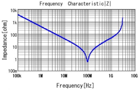
■ DE2B3KY471KA3BM02F |Z| DCOV, 20degC
