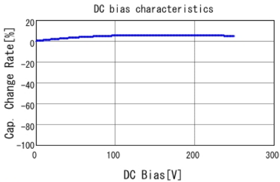
■ DE2B3KY471KA3BM02F C-DC bias capchange, 20.0degC, AC1
