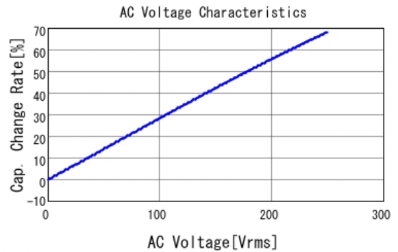
■ DE2B3KY471KB2BM01F C-AC Voltage capchange, DCOV, 20.0
