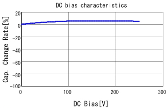
■ DE2B3KY471KB2BM01F C-DC bias capchange, 20.0degC, AC1
