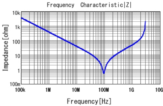
■ DE2B3KY471KB2BM01F |Z| DCOV, 20degC
