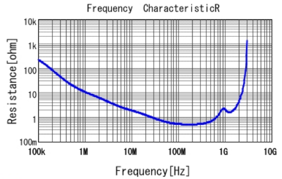
■ DE2B3KY471KB2BM01F R DCOV, 20degC
