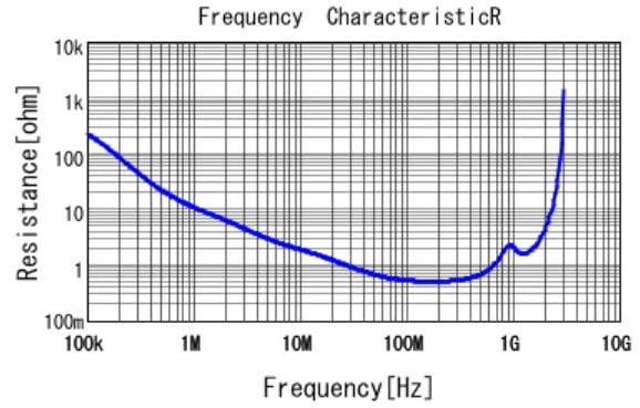
■ DE2B3KY471KN3AM02F R DCOV, 20degC
