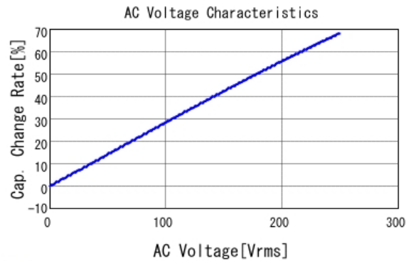
■ DE2B3KY471KN3AM02F C-AC Voltage capchange, DCOV, 20.0
