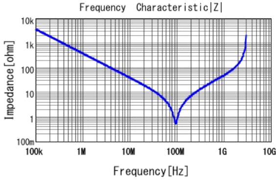
■ DE2B3KY471KN3AM02F |Z| DCOV, 20degC
