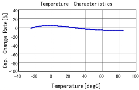
■ DE2B3KY471KN3AU02F C-Temp. capchange, DCOV, AC1Vrms
