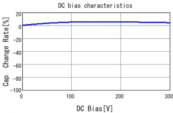
■ DE2B3KY471KN3AU02F C-DC bias capchange, 20.0degC, AC1
