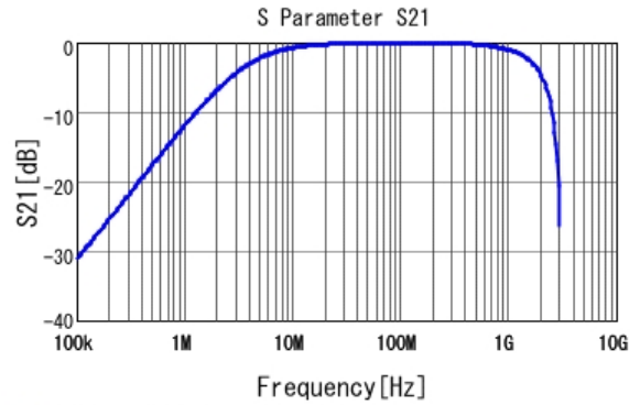
■ DE2B3KY471KN3AU02F S21 DCOV, 20degC
