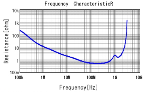
■ DE2B3KY471KN3AU02F R DCOV, 20degC
