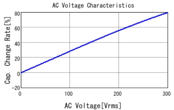
■ DE2B3KY471KN3AU02F C-AC Voltage capchange, DCOV, 20.0
