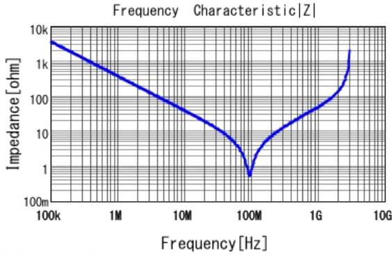
■ DE2B3KY471KN3AU02F |Z| DCOV, 20degC
