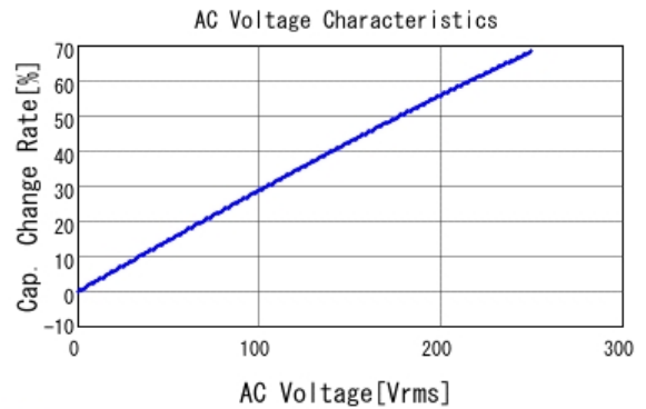
■ DE2B3KY681KN3AM02F C-AC Voltage capchange, DCOV, 20.0
