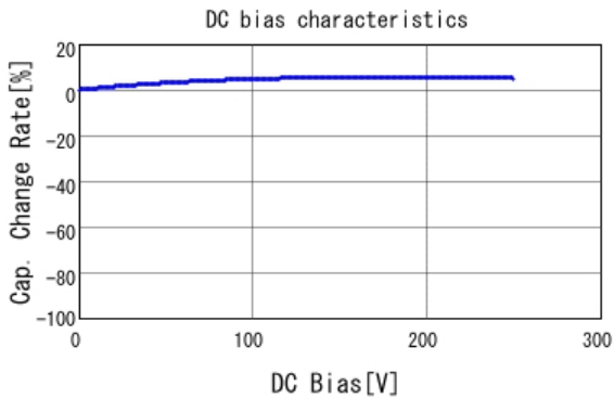
■ DE2B3KY681KN3AM02F C-DC bias capchange, 20.0degC, AC1
