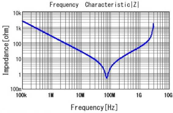
■ DE2B3KY681KN3AM02F |Z| DCOV, 20degC
