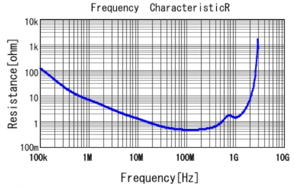
■ DE2B3KY681KN3AM02F R DCOV, 20degC
