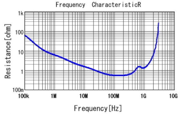
■ DE2E3KY102MA3BM02F R DCOV, 20degC
