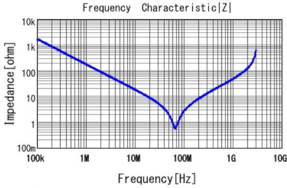
■ DE2E3KY102MA3BM02F |Z| DCOV, 20degC
