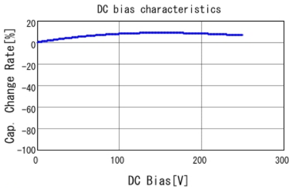
■ DE2E3KY102MA3BM02F C-DC bias capchange, 20.0degC, AC1
