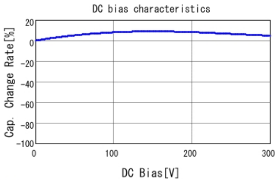
■ DE2E3KY102MA3BU02F C-DC bias capchange, 20.0degC, AC1
