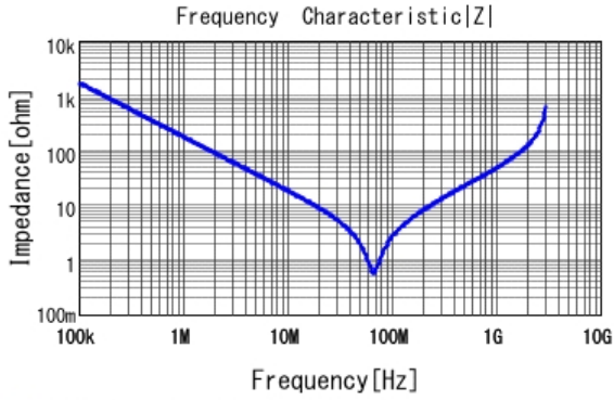
■ DE2E3KY102MN2AM01F |Z| DCOV, 20degC
