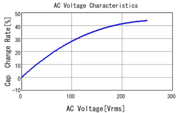
■ DE2E3KY102MN3AM02F C-AC Voltage capchange, DCOV, 20.0
