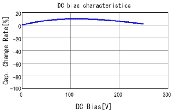
■ DE2E3KY152MA2BM01F C-DC bias capchange, 20.0degC, AC1
